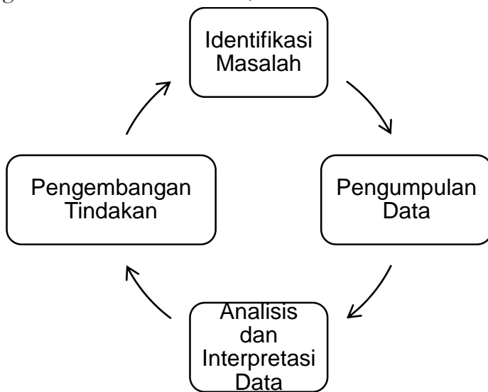
Gambar 5. Model Mills
