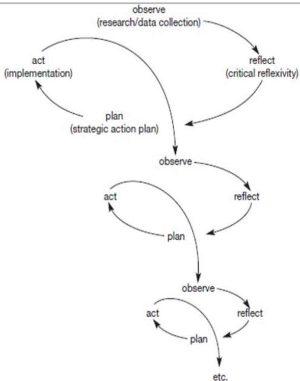
Gambar 8 Model O'Leary
