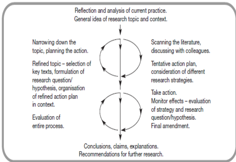
Gambar 10 Model Macintyre
